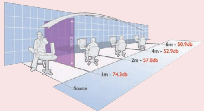
Sound Performance with a 1600mm high screen
